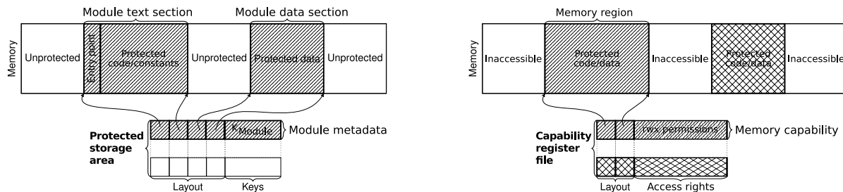
Figure 1 Fine-grained intra-address space isolation paradigms. Left: Sancus [5] uses the current value of the CPU’s program counter to distinguish a protected module (hatched) from untrusted code. The module’s data memory can only be accessed when executing in the corresponding text section , which can only be entered from a single predefined entry point . Software attestation is realized through a protected hardware storage area for metadata and cryptographic keys. Right: CHERI [6] relies on a dedicated CPU register file for unforgeable memory capabilities that provide read/write/execute permissions for individual memory regions (hatched). Flexible application protection domains are defined by deriving more restrictive capabilities at runtime.
